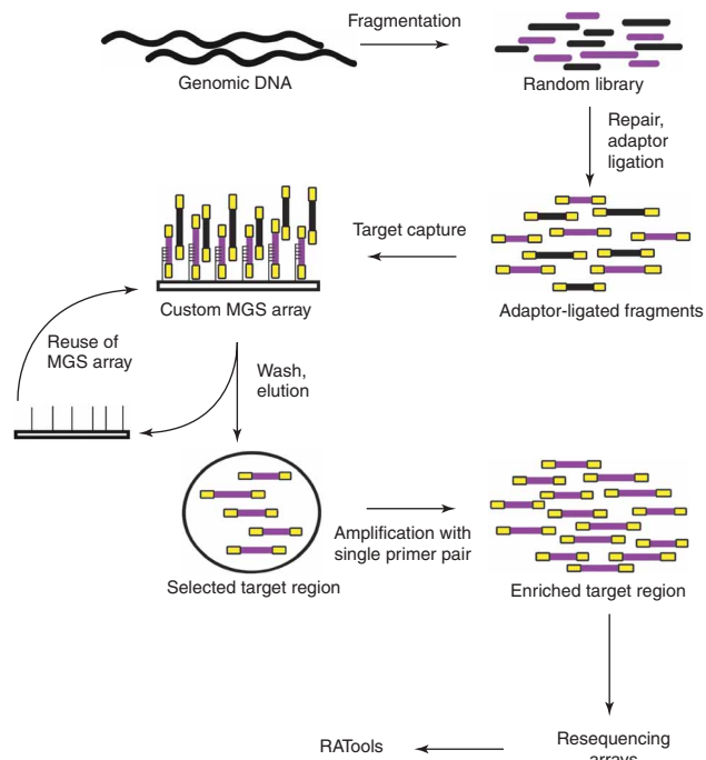
Figure 1 | Microarray-based genomic selection and resequencing of complex genomes. Sheared genomic fragments are repaired and ligated to generic adaptors. Hybridization to a custom designed high-density oligonucleotide microarray allows the capture of the target DNA regions. The selected target is eluted and amplified using a one-step PCR and a single primer pair per template. Amplified targets were resequenced with resequencing arrays and analyzed with RATools.
