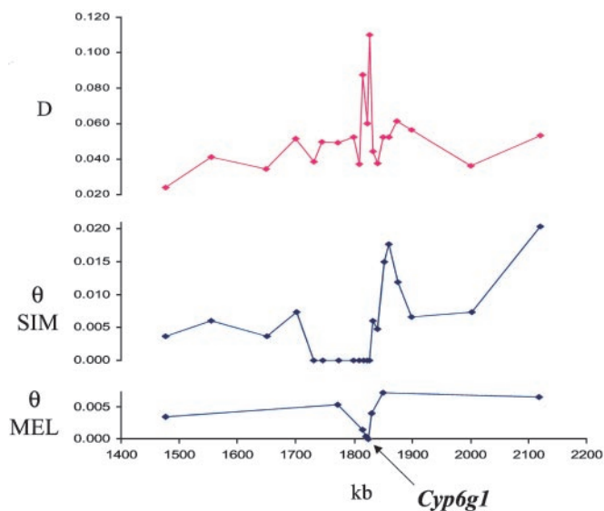
Fig. 2. Heterozygosity ( \theta ) and divergence ( D ) within and between California populations of D. simulans (SIM) and D. melanogaster (MEL) near the Cyp6g1 locus.
