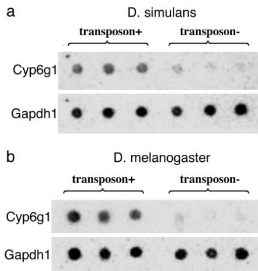
Fig. 4. Dot blots comparing levels of Cyp6g1 transcript in adult flies by using the control Gapdh1 (see Materials and Methods ). (a) The first three D. simulans dots are from the Californian lines CS1, CS2, and CS3, whereas the last three are from the African lines AS1, AS2, and AS3. (b) The first two D. melanogaster dots and the fourth dot are from the Californian lines CM1, CM2, and CM3, whereas the third dot and the fifth and sixth dots are from the African lines AM3, AM2, and AM5.
