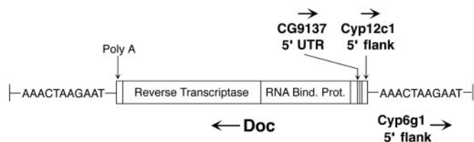
Fig. 3. The structure of the D. simulans Doc insertion. The genomic sequence duplicated by Doc is shown to either side. Horizontal arrows represent the direction of transcription or, for noncoding sequence, the direction of transcription of the associated gene.
