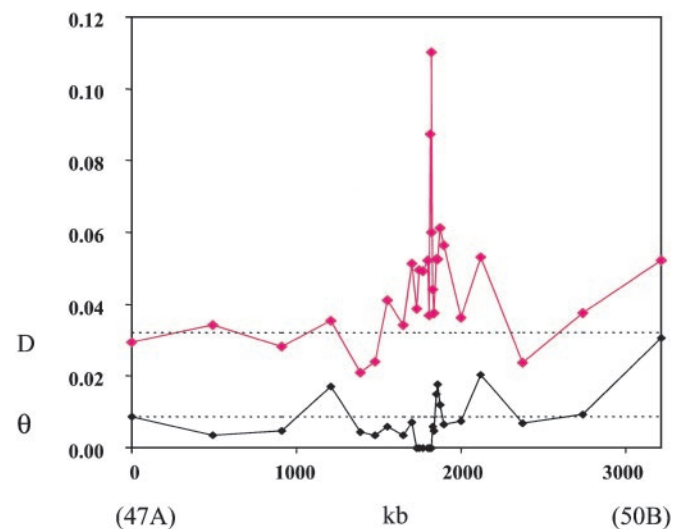
Fig. 1. Heterozygosity ( \theta ) and divergence ( D ) across chromosome 2R, cytological position 47A to 50B, in California D. simulans . Position in kb is relative to the first locus. Dashed lines represent an independent estimate of average values for the species (11).
